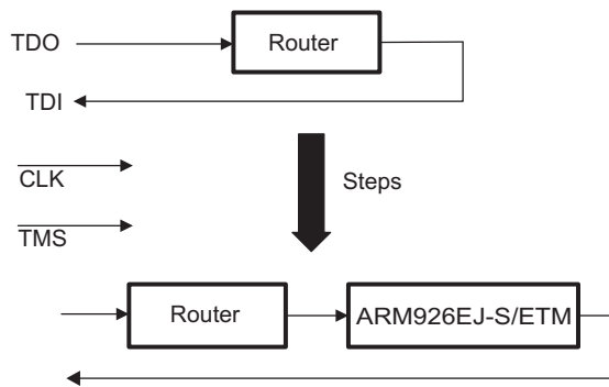
Figure 6-67. Adding ARM926EJ-S to the scan chain
